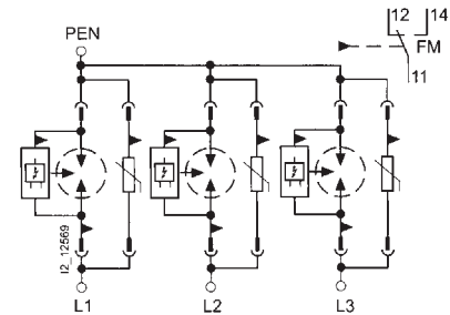
5SD7 443-1
